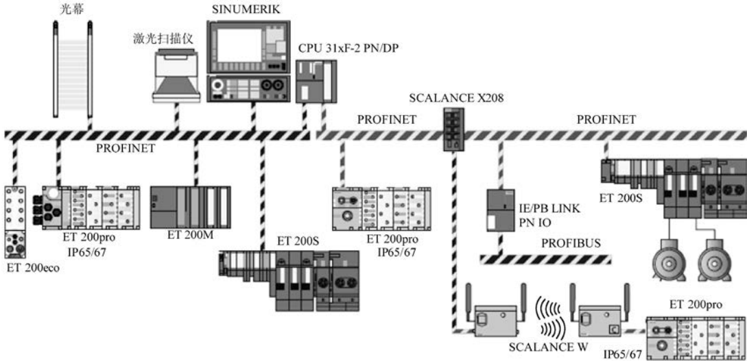
图 2-7 PROFIsafe
