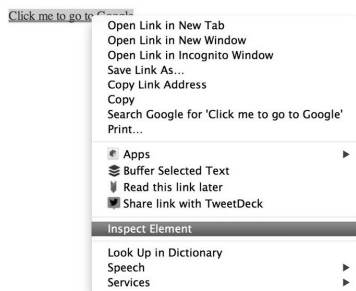
图8-3 Inspect Element
