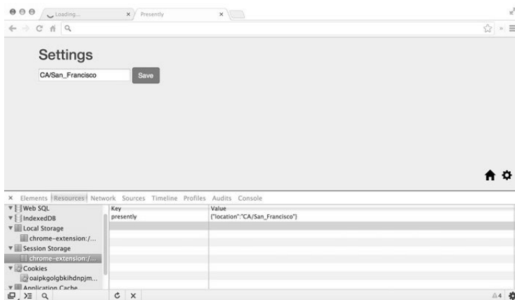
图31-9 sessionStorage
