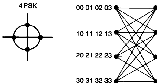
图7-19 2STTC, 4PSK, 4状态, 2 bit/s/Hz
