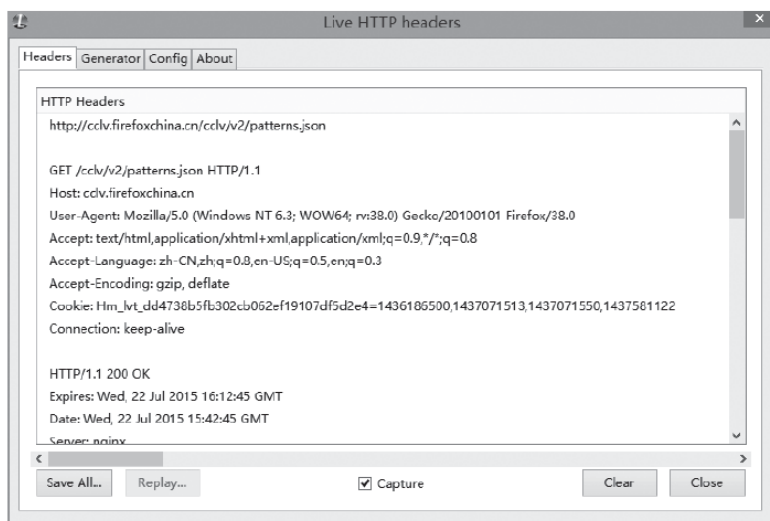
图4-7 Live HTTP headers
