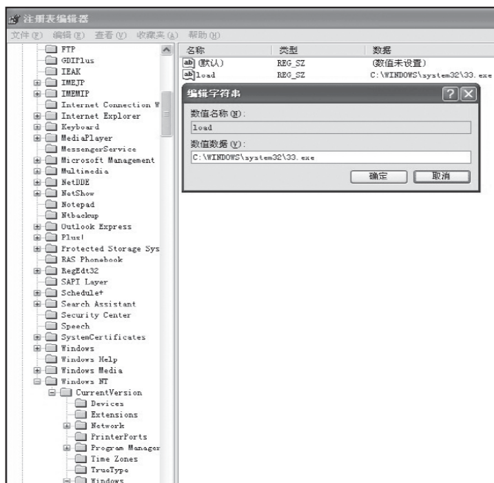
图9-58 regedit
