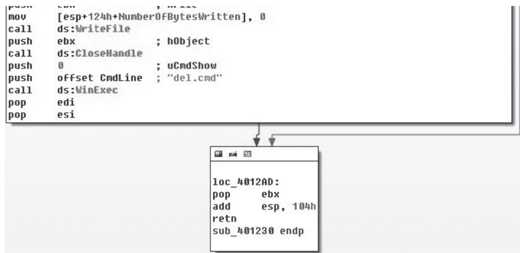
图9-53 CreateFileA ( 2 )
