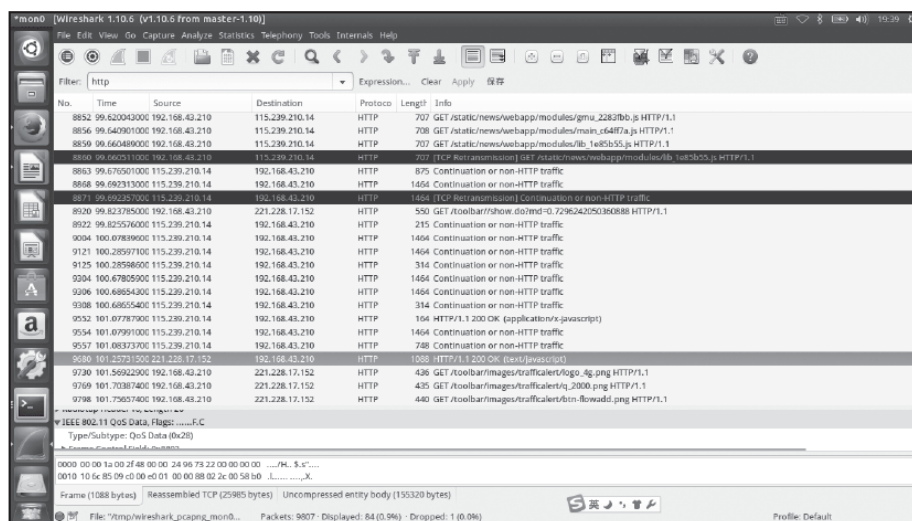
图5-13 Wireshark的http筛选器效果
