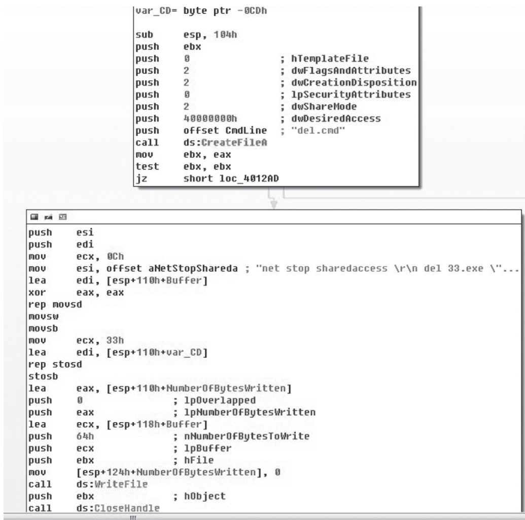
图9-52 CreateFileA ( 1 )
