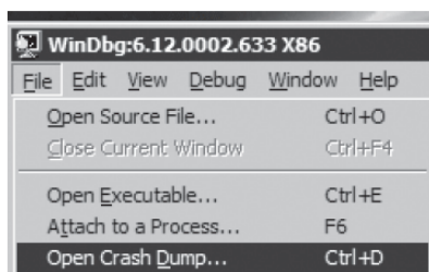
图9-64 File菜单
