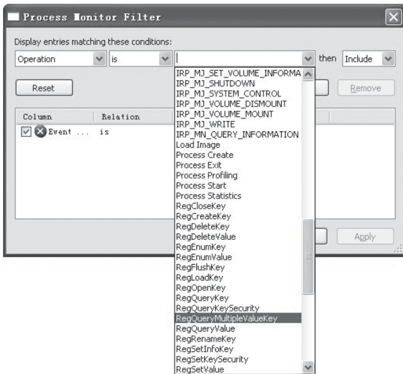
图9-22 Filter过滤
