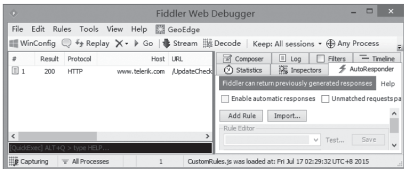
图4-3 Fiddler
