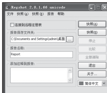
图9-24 Regshot
