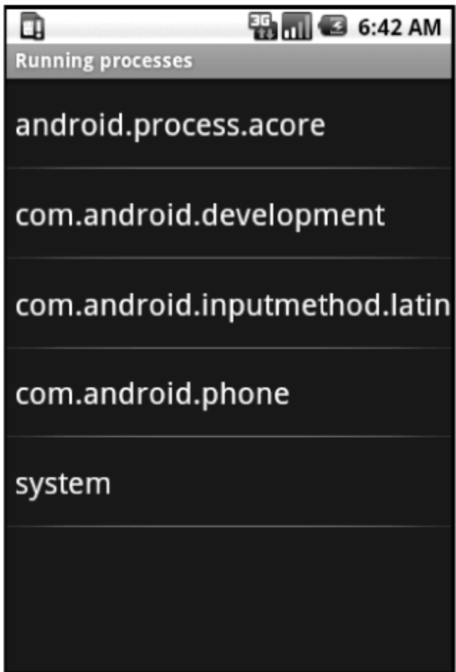
图 4.18 Running processes
