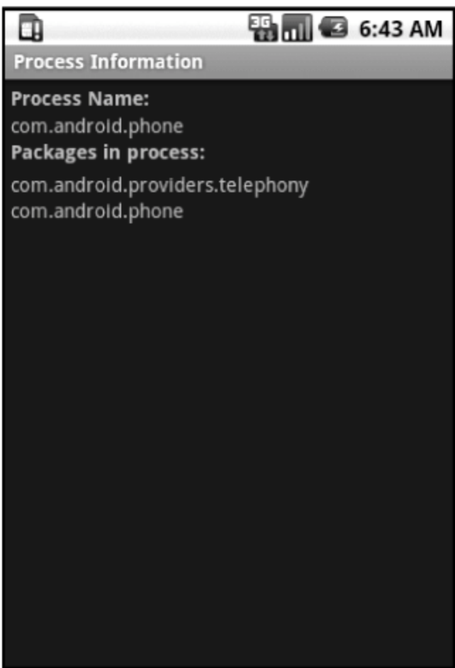
图 4.18 Running processes
