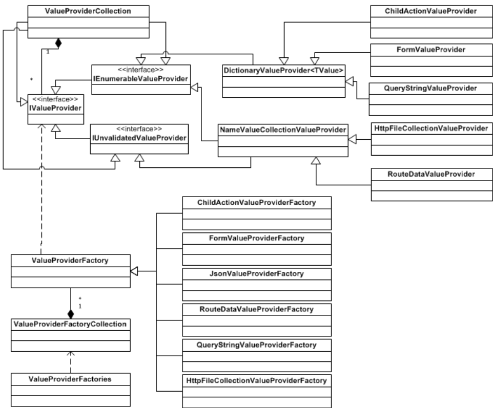
图 5-6 ValueProvider-ValueProviderFactory-ValueProviderFactories
