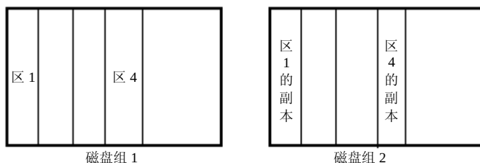
图 8-4 常规冗余 (Normal Redundancy)
