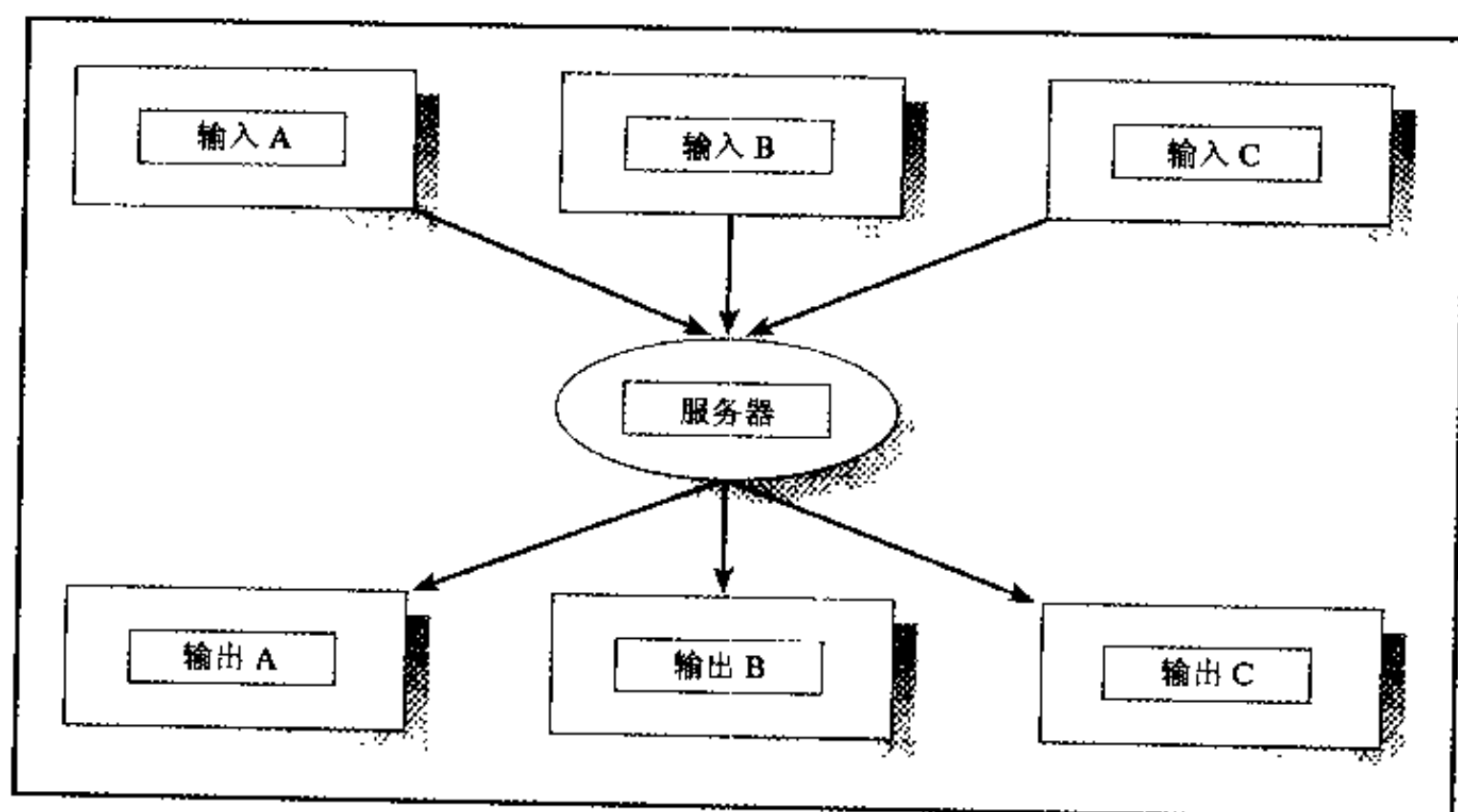
图 4.3 Client/Server
