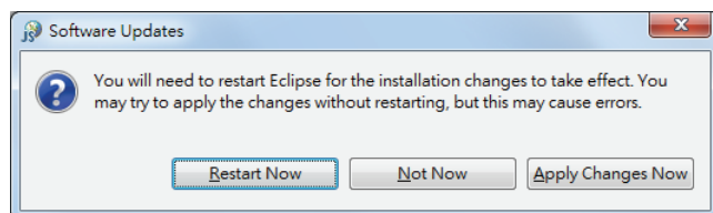
图3-14 Restart Now
