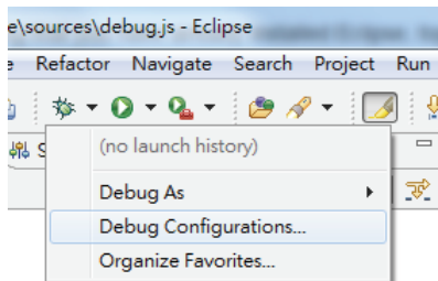
图3-16 Debug Configurations...
