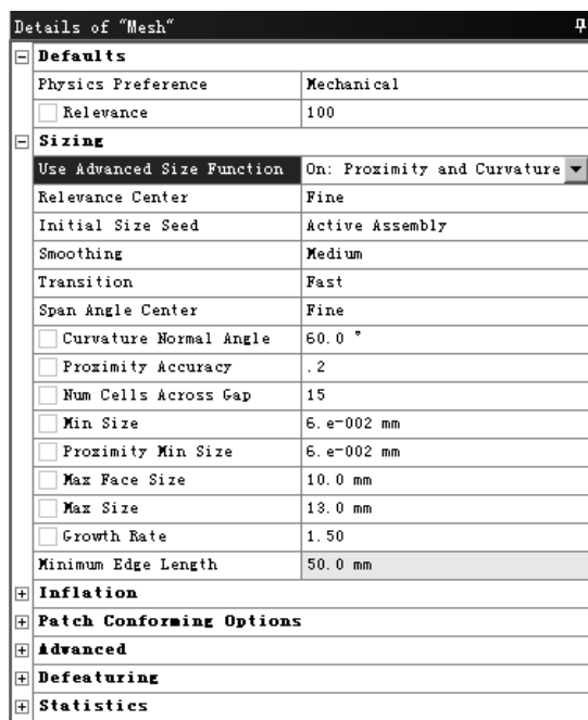
图 4.2.13 “Details of ‘Mesh’”对话框
