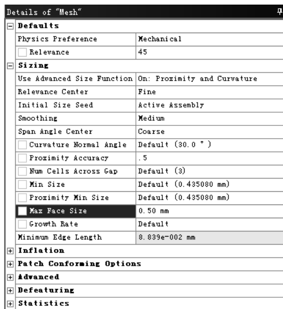
图 9.5.9 “Details of ‘Mesh’”对话框
