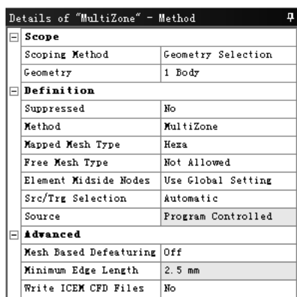
图 4.3.14 “Details of ‘MultiZone Method’ -Method”对话框
