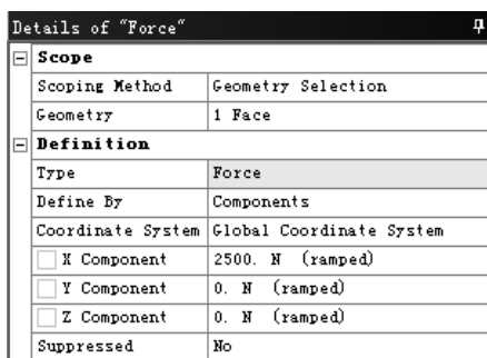
图 9.5.17 “Details of ‘Force’”对话框
