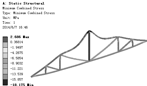
b) Minimum Combined Stress
