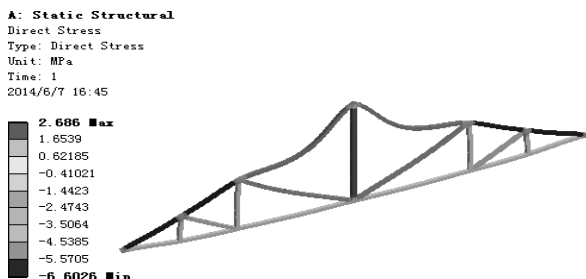
a) Direct Stress
