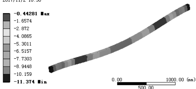
b) Minimum Combined Stress
