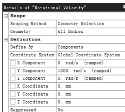
图 4.2.7 “Details of ‘Rotational Velocity’”对话框
