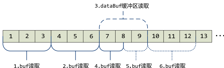
图 5-11 readWithBounceBuffer()示例
